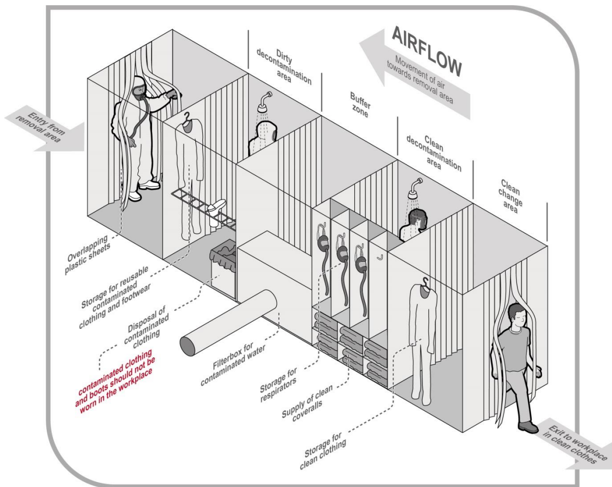
Figure 4 Decontamination unit
